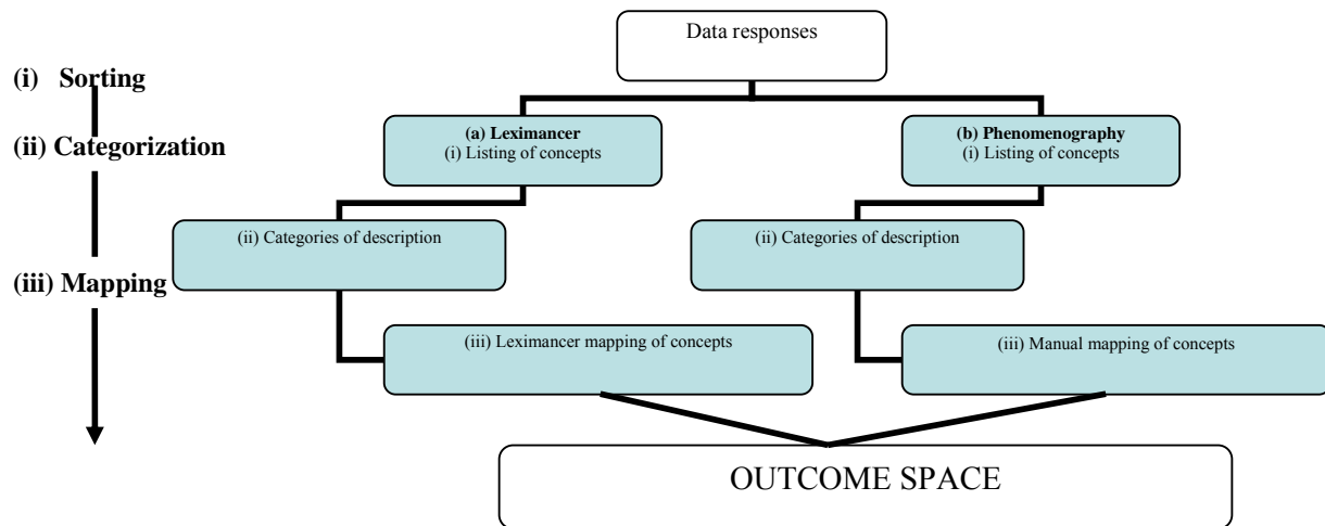
Figure 1. Analysis processes
